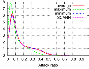
(b) PDF of attack ratio for rejected communities (large probability for low attack ratio is better)
