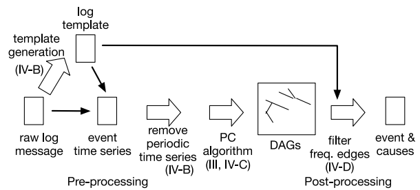
Fig. 2. Processing flow.
