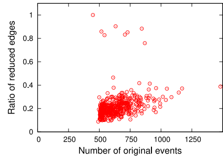
Fig. 6. Preprocessing: edge reduction.
